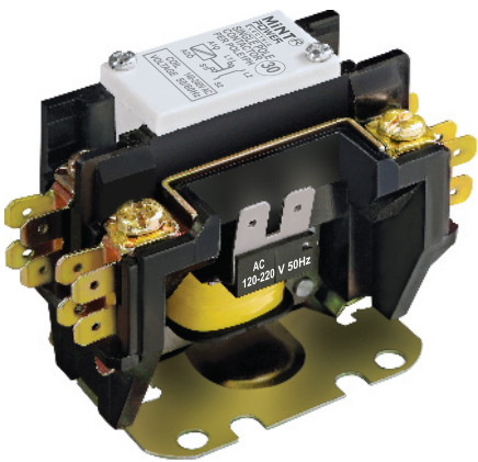
1-POLE
